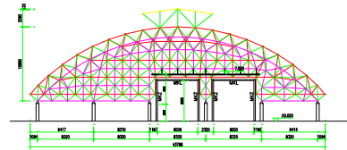
Awning layout Plan 1 MK2, MK3, MK4, MK5
