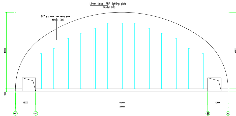
Axis 1 Building elevation
