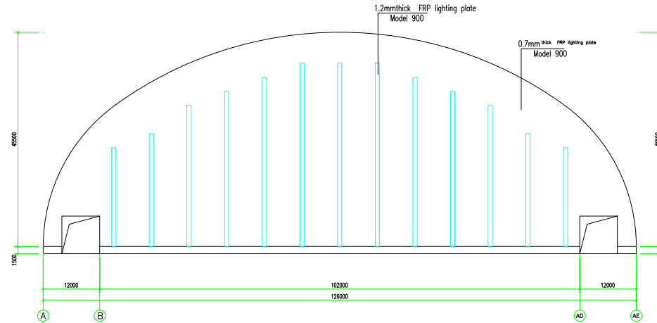
Axis 109 building elevation
