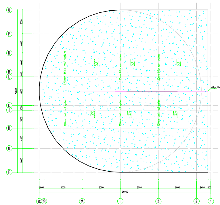
Grid roof layout plan
