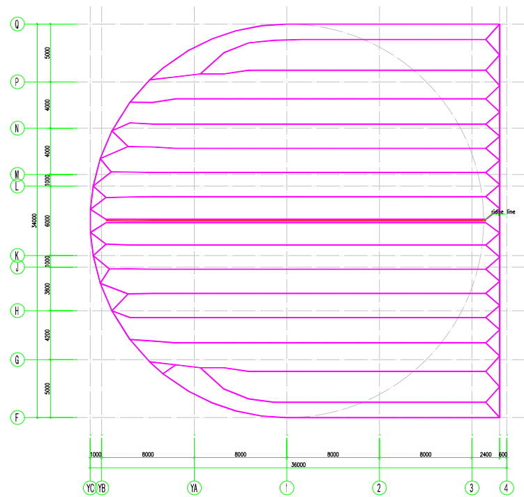
layout of roof girder
